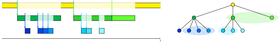
Fig. 1 Gantt chart of the regions (left) and the interruption tree (right) generated by the region algorithm (color figure online)
